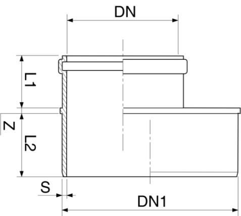
Eccentric female/male reducer -
