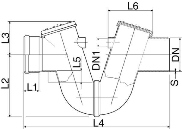
Trap with register male/female -
